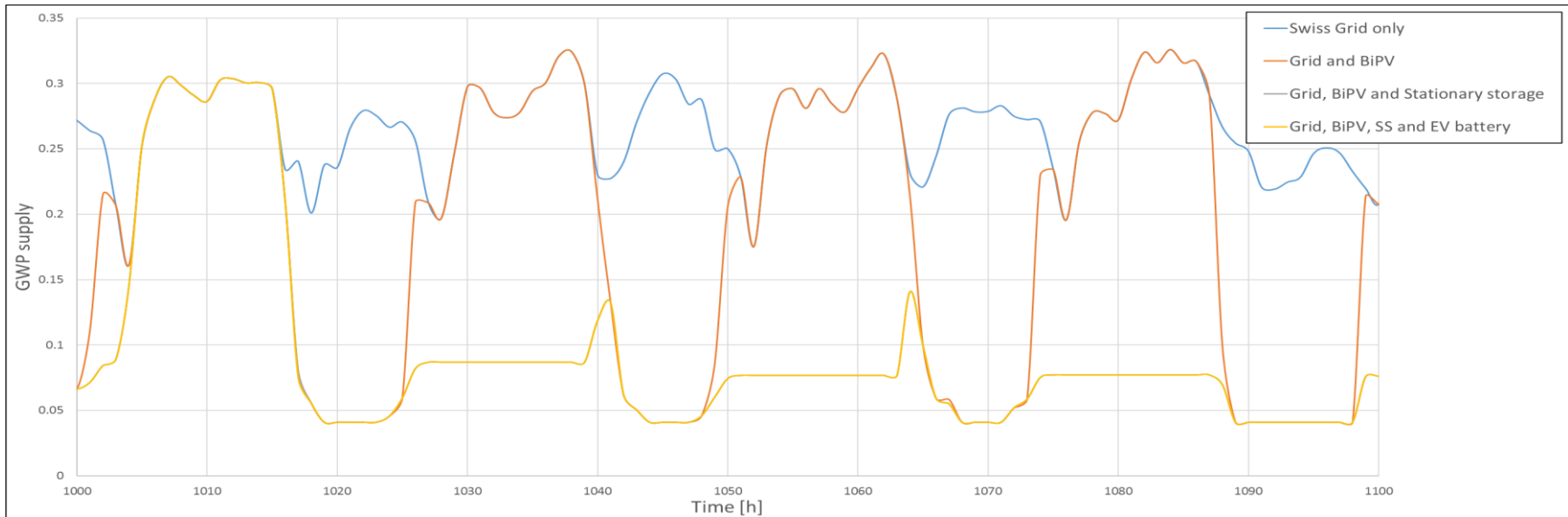
Figure 4. Hourly GWP supply on a 100 hour range
