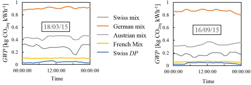
Figure 1. GWP of the contributors to the Swiss mix (DP: domestic production) [1]
