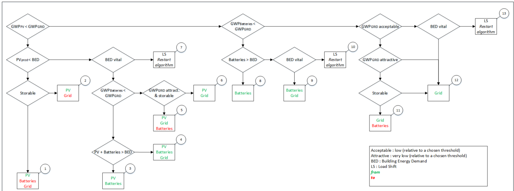
Figure 3. Algorithm's decision tree
